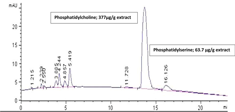
Fig. 1. HPLC chromatogram of Arabic gum. For HPLC analysis, samples (20 mL) were injected and eluted using the degassed mobile phase, which was supplied at a flow rate of 0.80 mL/min and consisted of acetonitrile, methanol, and 85 % phosphoric acid (96:3:1, v/v/v). Using comparable phospholipid standards, the concentration of each sample was determined while the effluent was being monitored at a wavelength of 203 nm. The source of the standard (GSH: 200–725–4) was the Sigma Chemical Company located in St. Louis, MO, USA.
